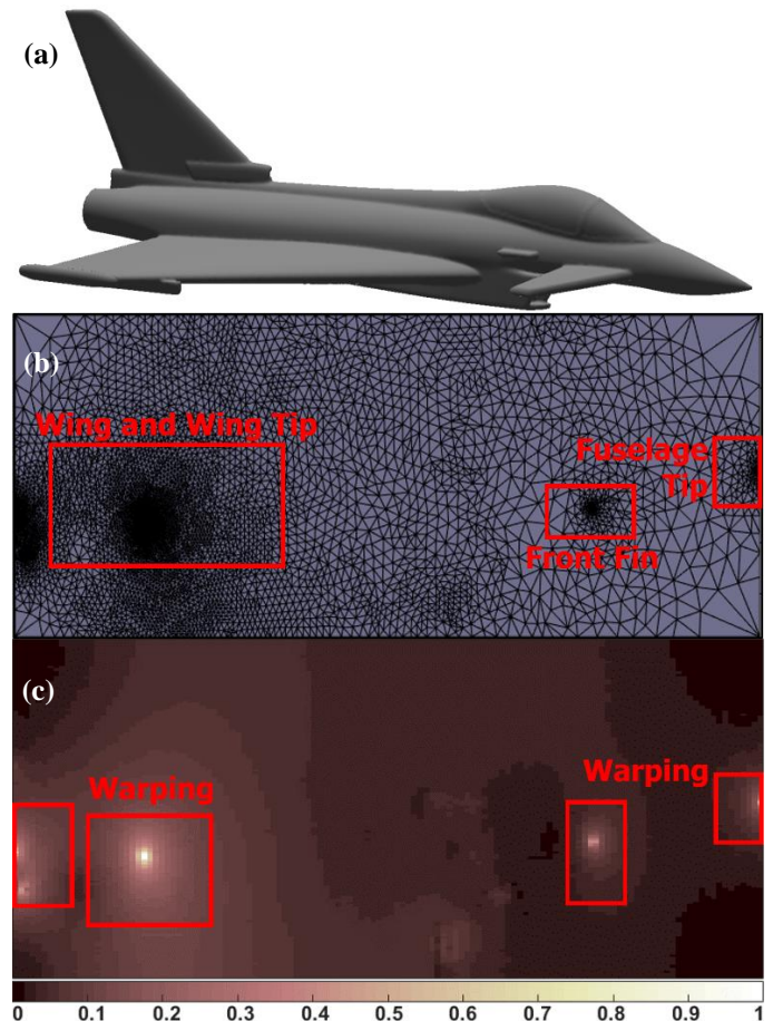
Fig. 4. (a) Initial fighter jet surface. (b) Triangle mesh of fighter jet cut and conformally flattened to the plane with highly warped areas boxed in red. (c) Refinement indicator (normalized) for each quadrilateral element demonstrating high degree of warping at fighter jet fin, wing, and fuselage tip when uniform sampling is used.
