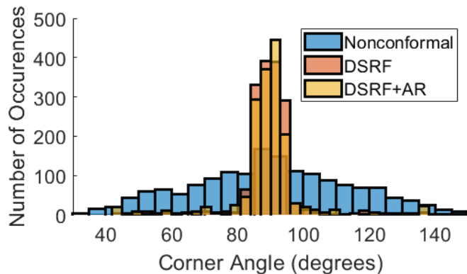
Fig. 3. Corner angle histograms for 20 \times 20 structured quadrilateral meshes show in Fig 2. Nonconformal mesh has a poor corner angle distribution while meshes obtained using DSRF have distributions concentrated closely around 90 degrees.
