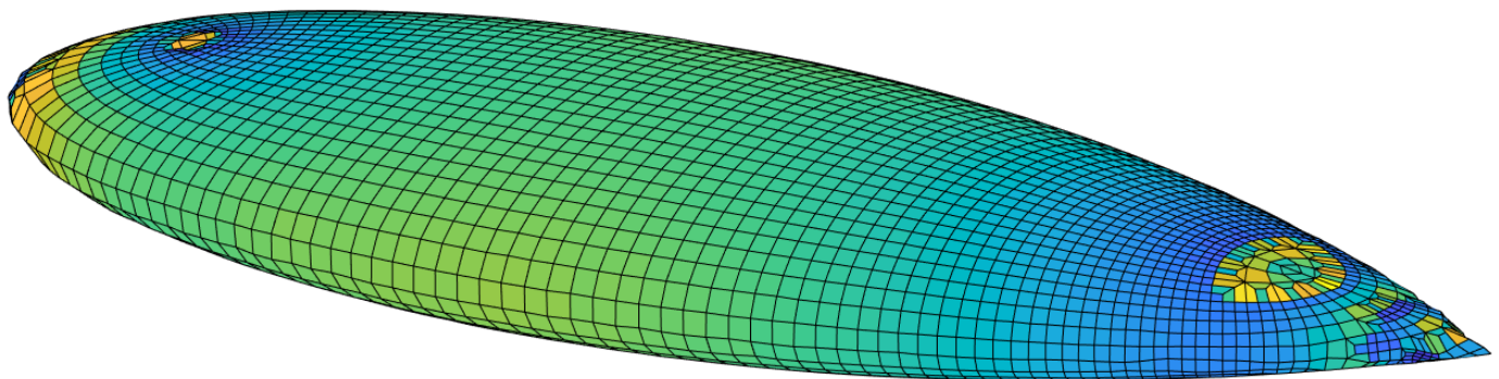
Fig. 20. NASA almond model containing 1544 1 st -order continuous quadrilateral elements based on the adaptive refinement from Fig. 8.
