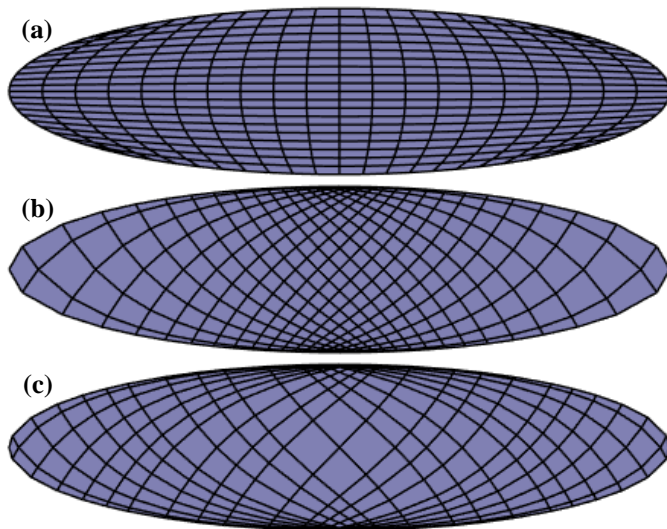
Fig. 2. 20 \times 20 structured quadrilateral meshes mapped to an ellipsoid using (a) a nonconformal mapping; (b) a conformal mapping by DSRF, parametric domain sampling shown Fig. 1(b); and (c) a conformal mapping using DSRF with adaptive refinement, parametric domain sampling shown Fig. 1(c), to capture more detail in regions of high curvature.
