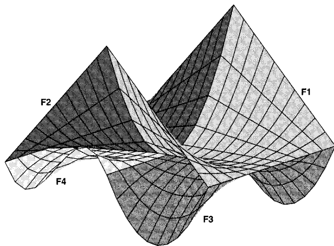
Fig. 3. Four characteristic terms of polynomial expansion in (11) defined on two adjacent bilinear surfaces. Function F1 is defined on surface 1 with i = 1 and j = 2 , F2 is defined on surface 2 with i = 0 and j = 2 , F3 is defined on surface 1 with i = 2 and j = 2 , F4 is defined on surface 2 with i = 3 and j = 3 . F1 and F2 are the same along the common edge, and the corresponding polynomial coefficients are common for the two surfaces. F3 and F4 are zero along the common edge.
