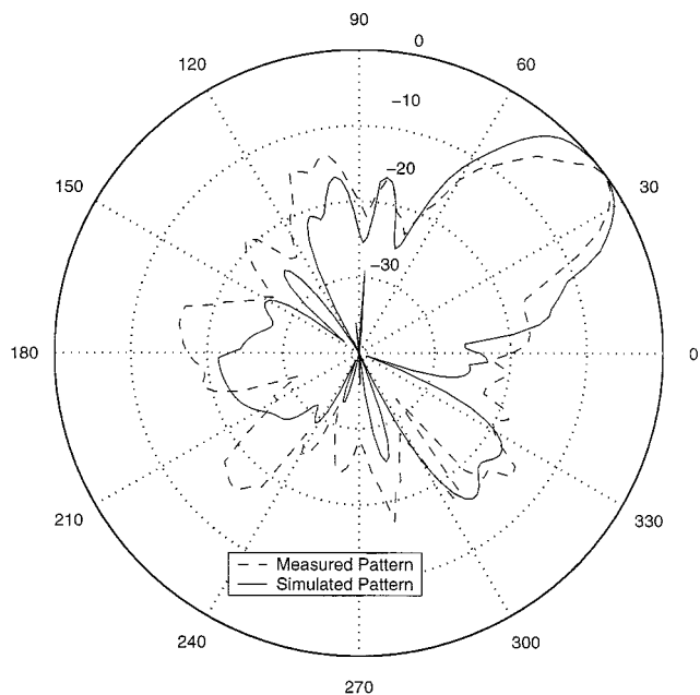
Fig. 5. Simulated and measured radiation pattern of antenna in Fig. 4 in plane \phi = 0^\circ .
