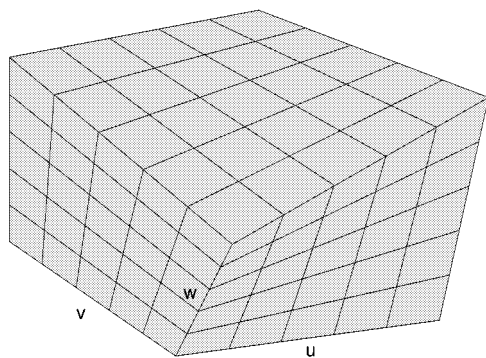
Fig. 2. Trilinear hexahedron.
