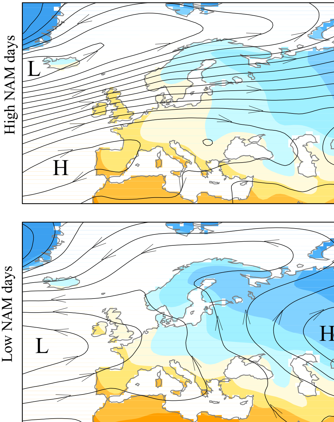
Composite maps of SAT (shading) and SLP (contours) based on daily JFM data, 1958-1997. Contour intervals 5^{\circ} C (blue shades indicate values < 0^{\circ} C and 3 mb for SLP).
